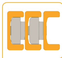
Montante triplex con cuscinetti Triplex profile with bearing
